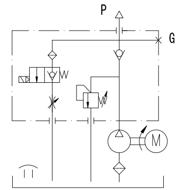
HYDRAULIC CIRCUIT 101
